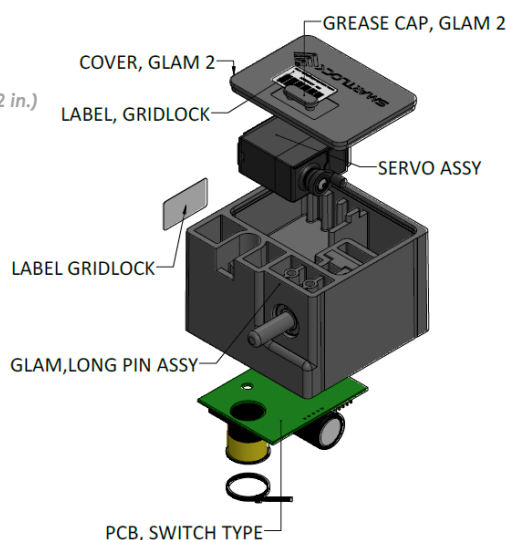
ISOMETRIC (EXPLODED) VIEW:
